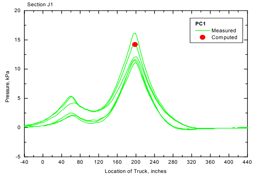
Figure 4 - Pressure at Interface between Base and Subgrade
