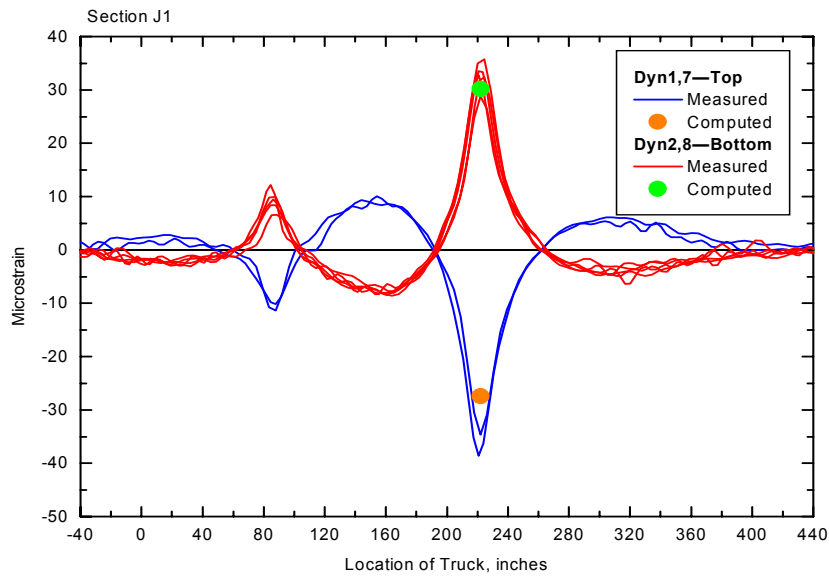
Figure 3 - Pavement Strain
