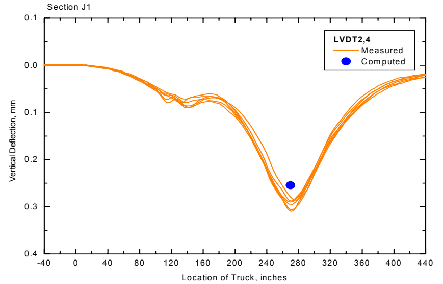
Figure 2 - Vertical Deflection of Pavement
